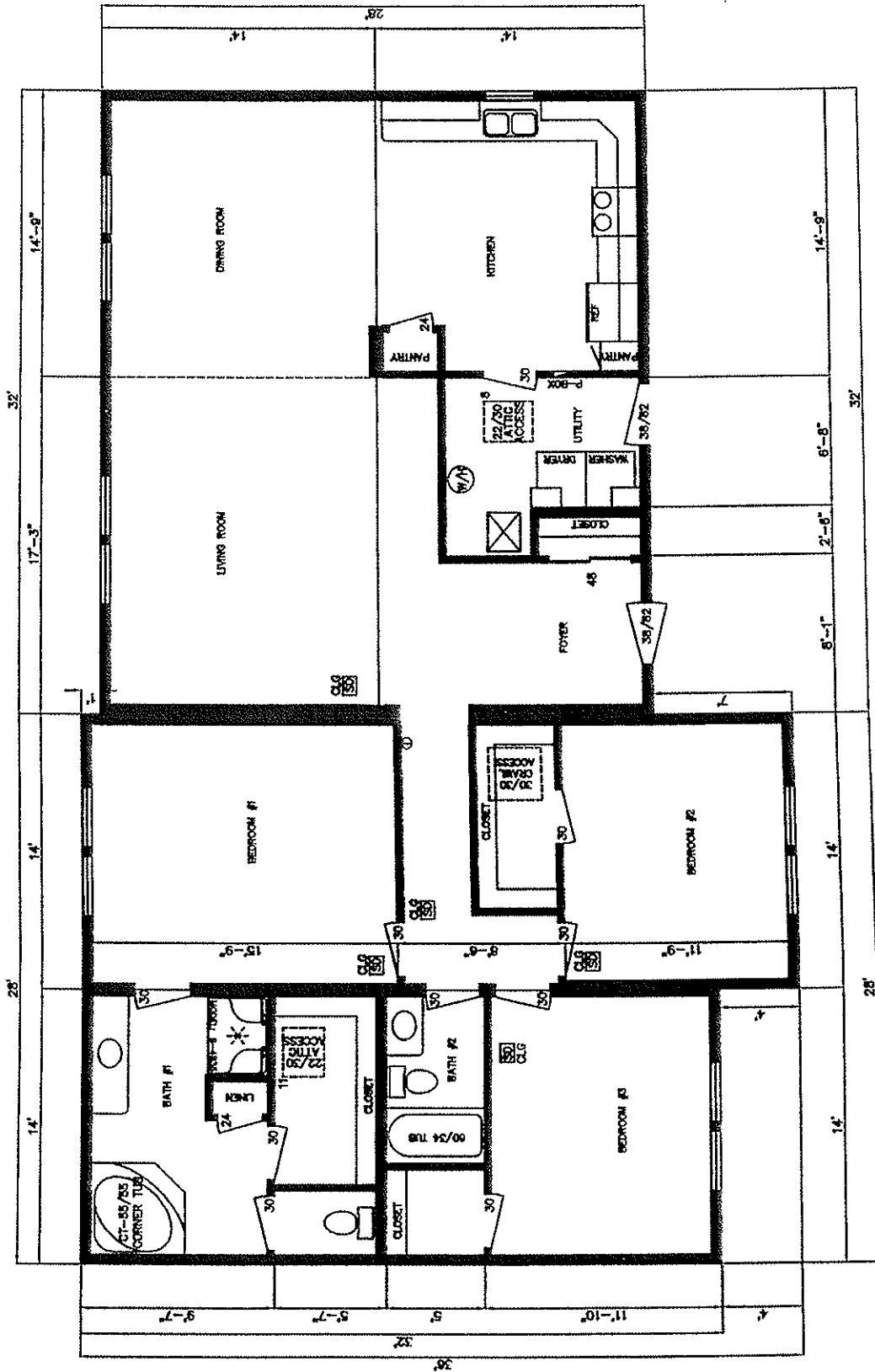
Model: CAMDEN Floor Size: 28'-0" X 36'-0" / 32'-0" (2,301 sq ft)
